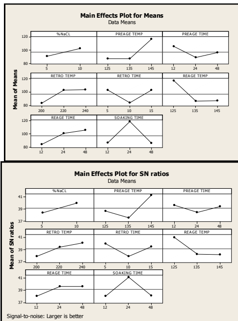
Fig. 6: Main effects plot for Means and S/N ratios of 10% SiC
