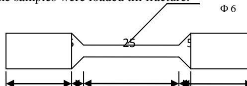
Fig 3: Tensile test specimen
