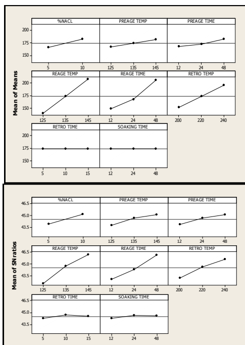
Fig. 7: Main effects plot for Means and S/N ratios of 15% SiC
