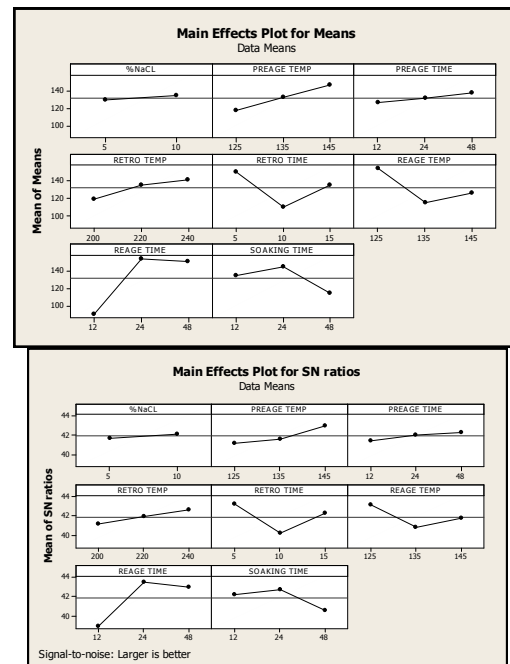
Fig. 5: Main effects plot for Means and S/N ratios of 5% SiC
